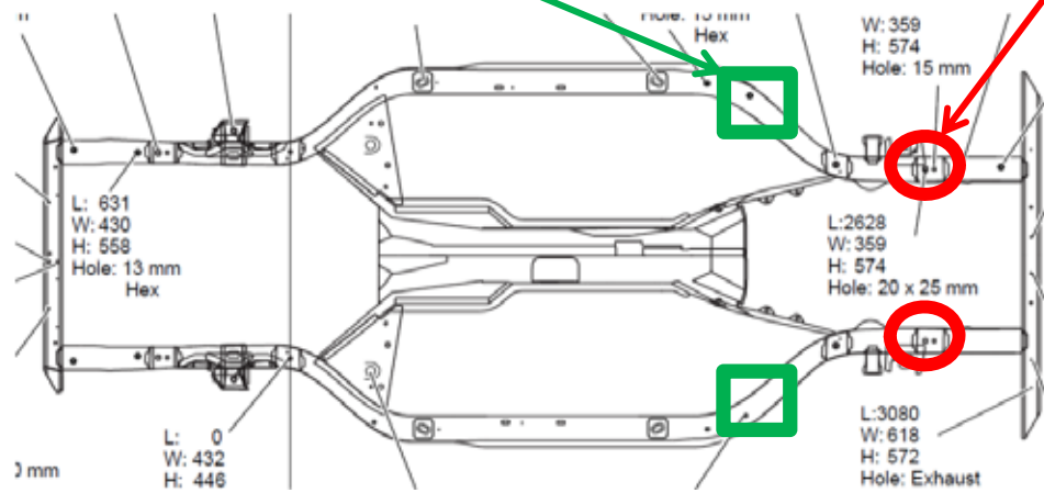
On the frame behind the B pillar, access through gas tank opening
