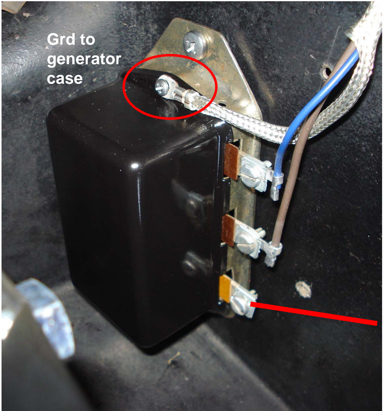
Wiring for 1960 Voltage Regulator
