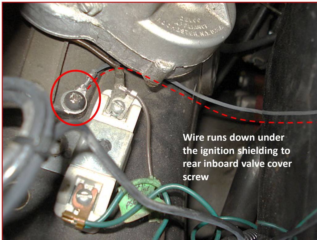
Note: all ground wires above are black. The colored lines are for tracing the routing.
