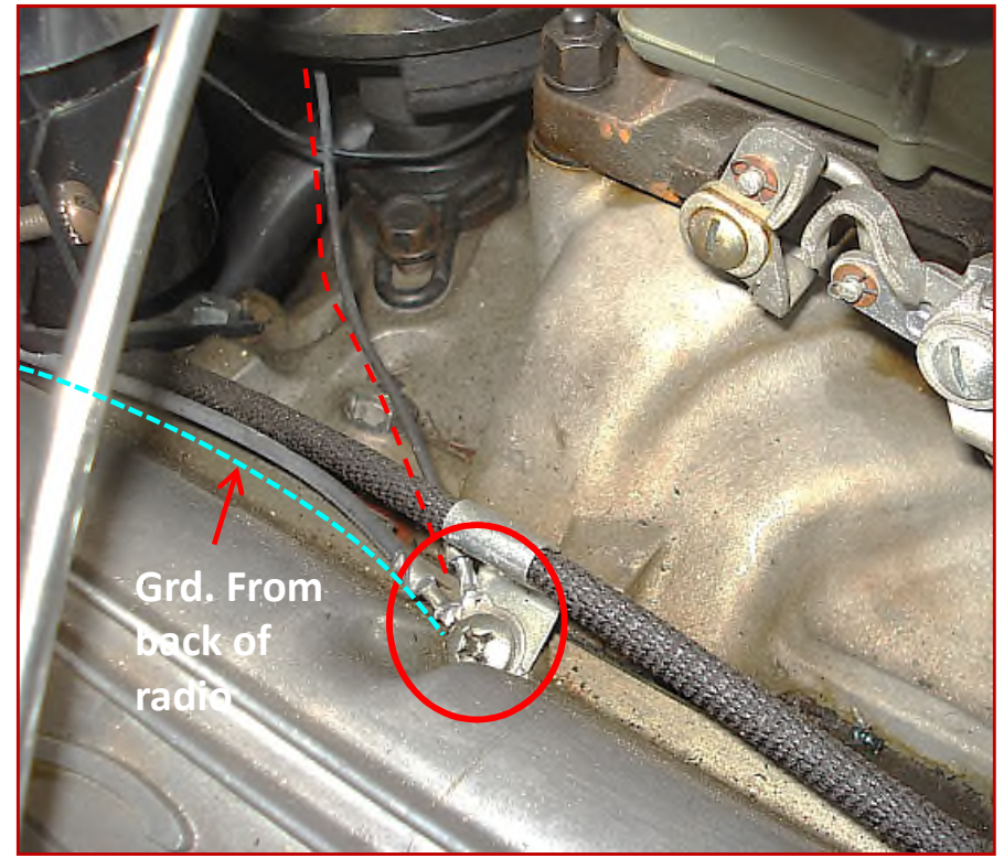
Note: all ground wires above are black. The colored lines are for tracing the routing.
