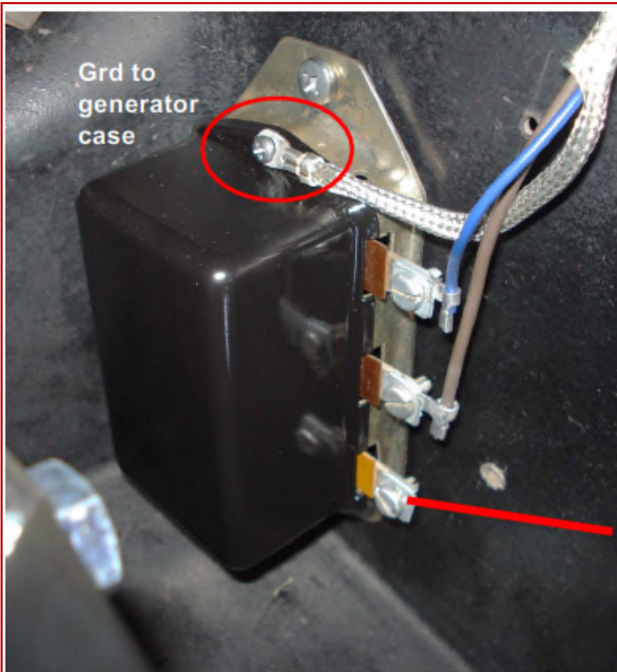
Wiring for 1960 Voltage Regulator
