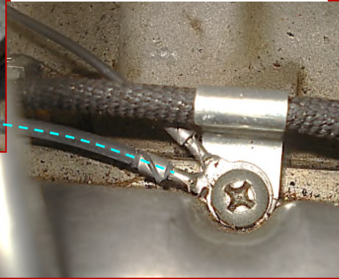
Wiper and radio grounds to psgr side valve cover
