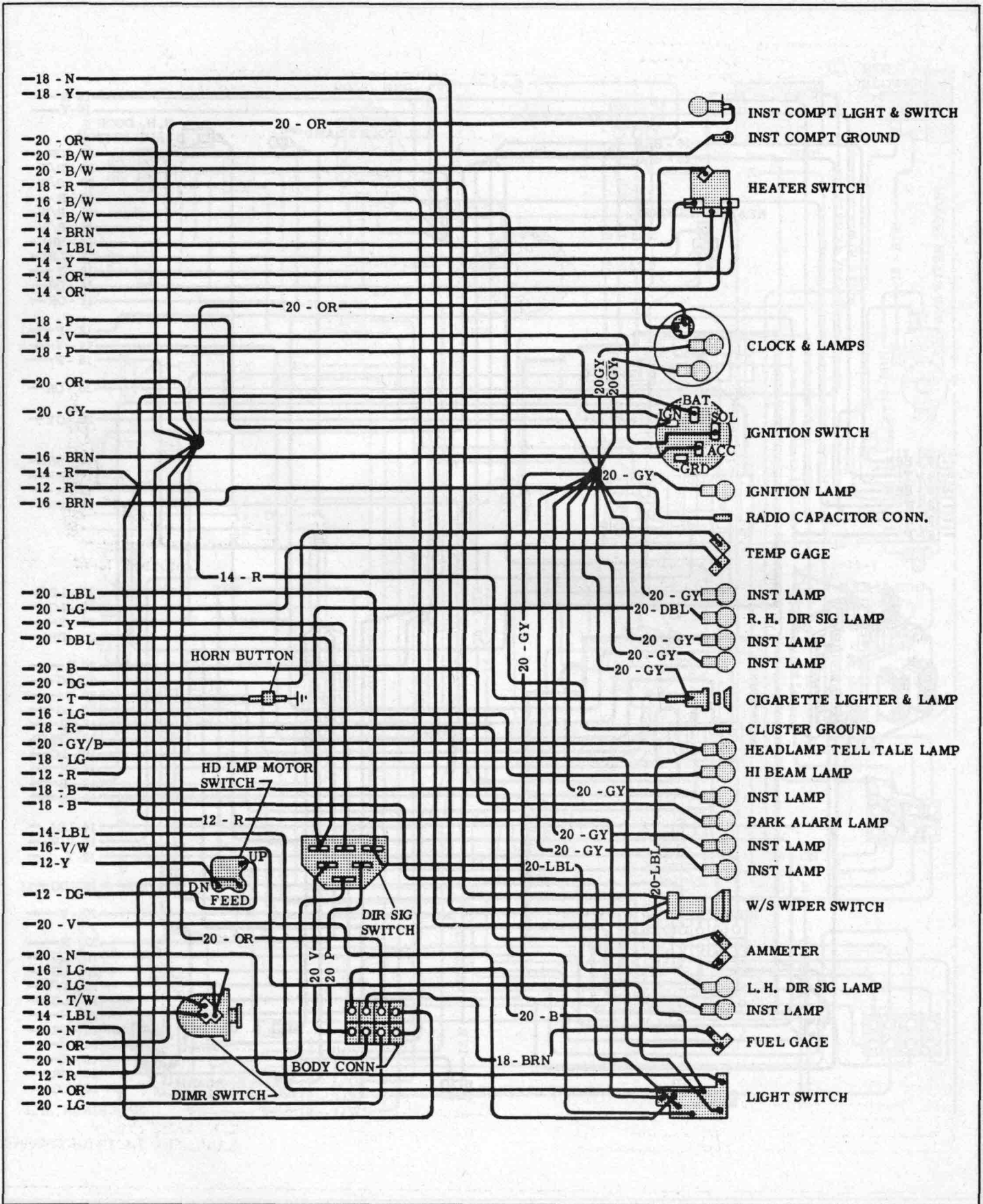
Fig. 41c—Instrument Panel Wiring
