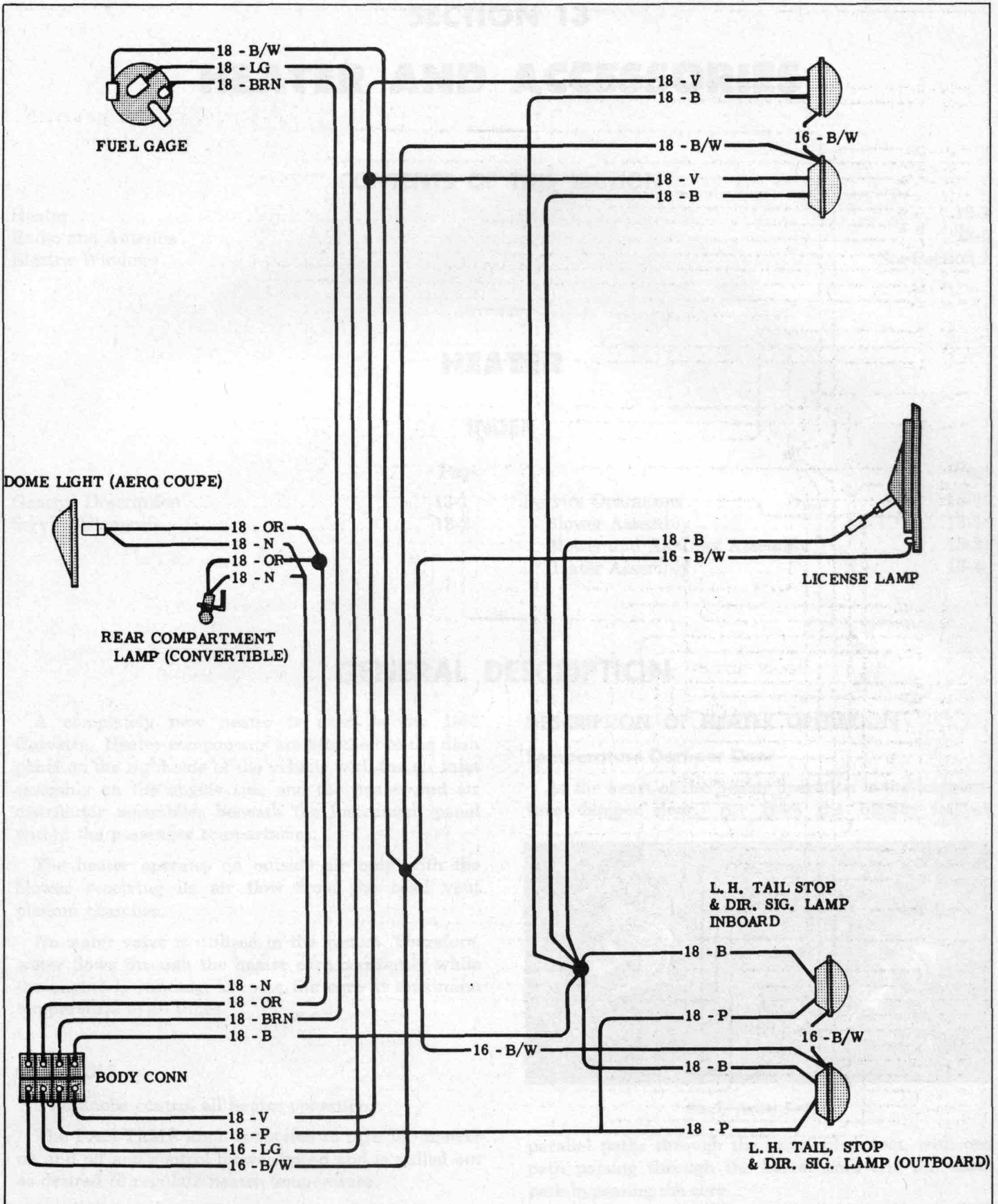
Fig. 41d—Body and Tail Lamp Wiring
