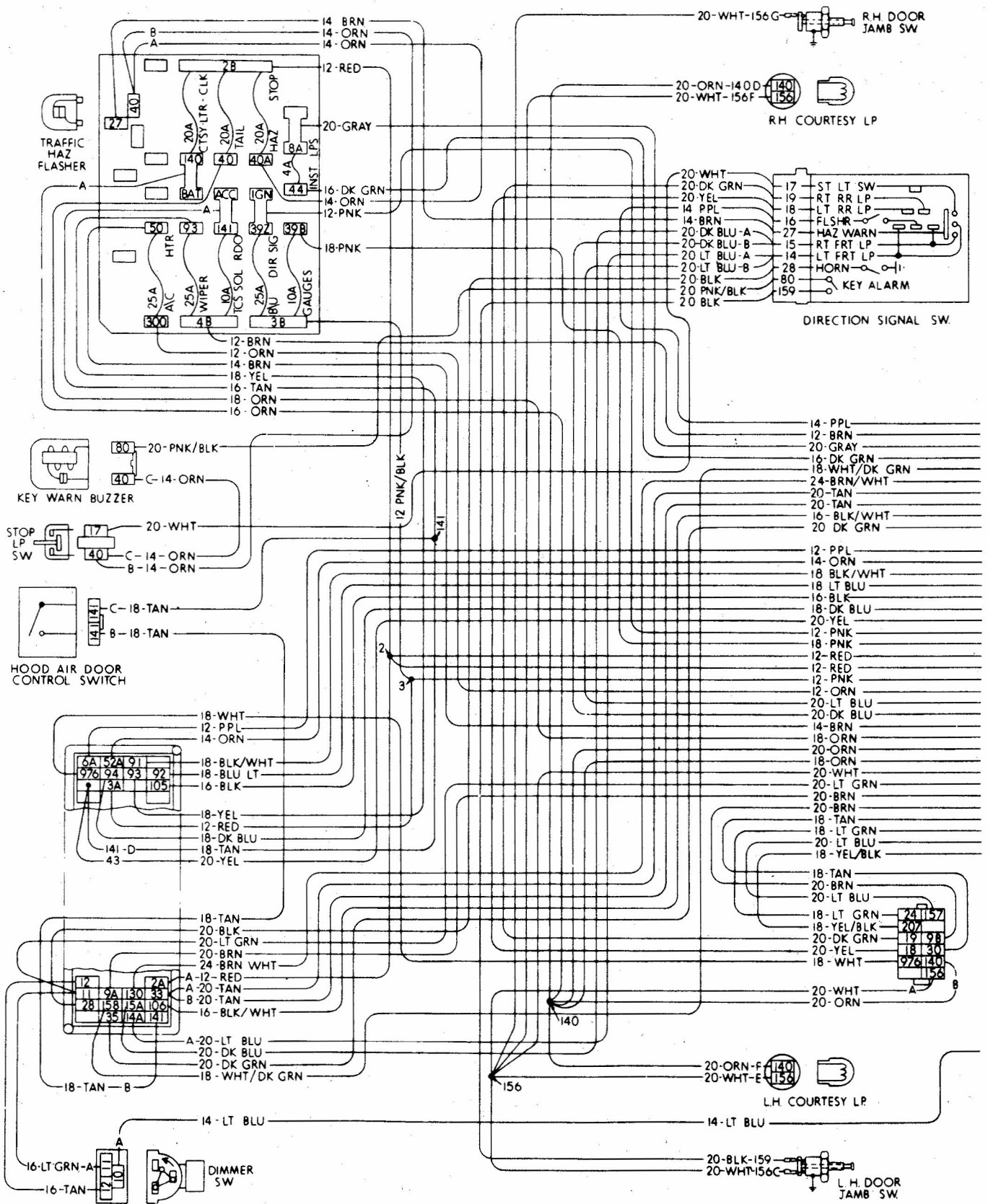
Wiring diagram for 1973 models - instrument panel (1 of 2)
