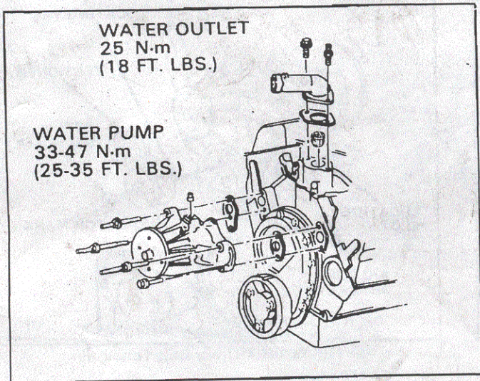
Figure 6B-2 Water Pump
