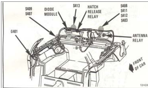
Figure A - Rear Cargo Compartment
