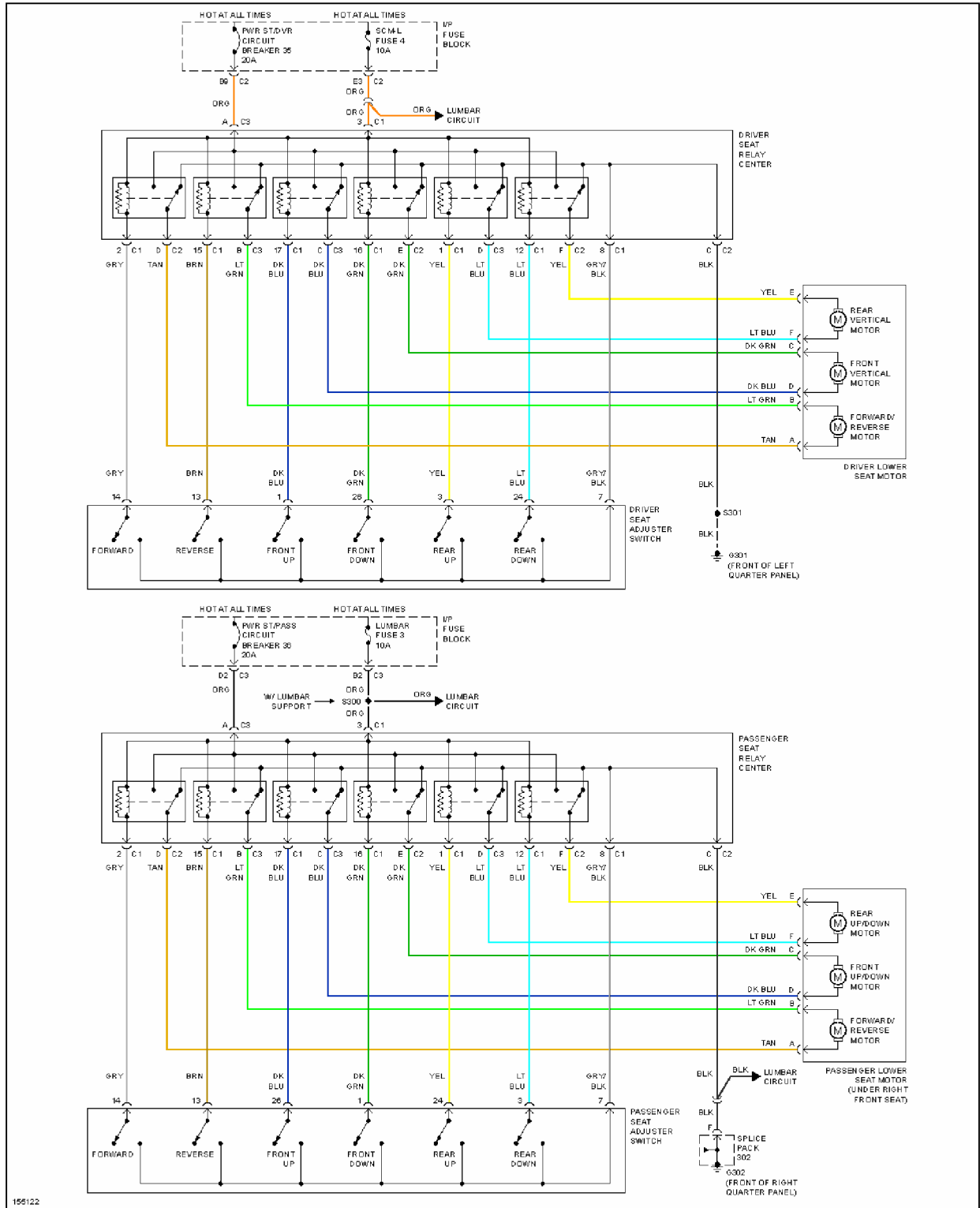
Fig. 38: 6-Way Power Seat Circuit
