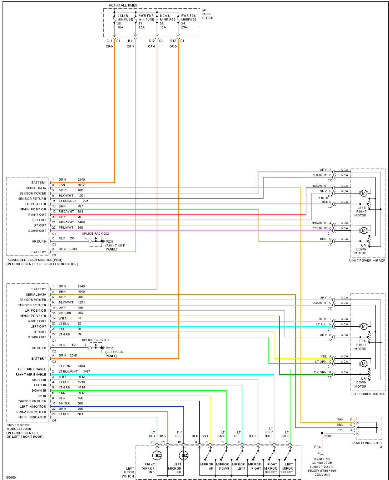
Fig. 37: Power Mirrors Circuit
