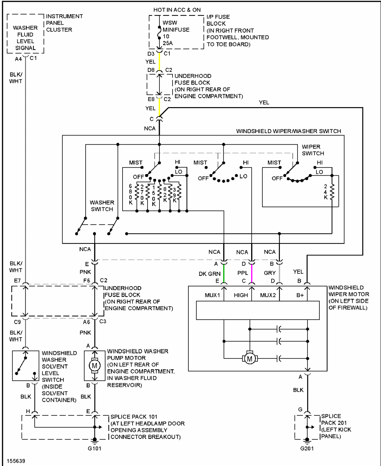
Fig. 52: Wiper/Washer Circuit
