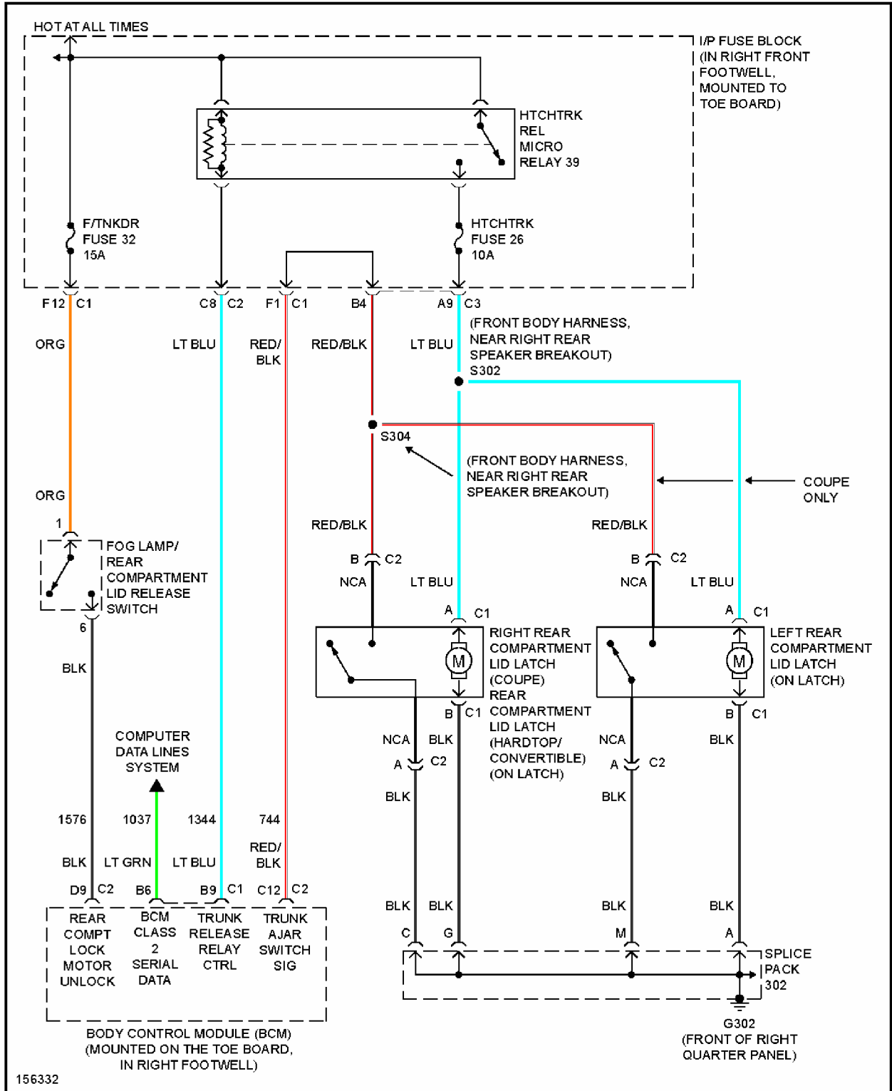
Fig. 50: Hatch Release Circuit
