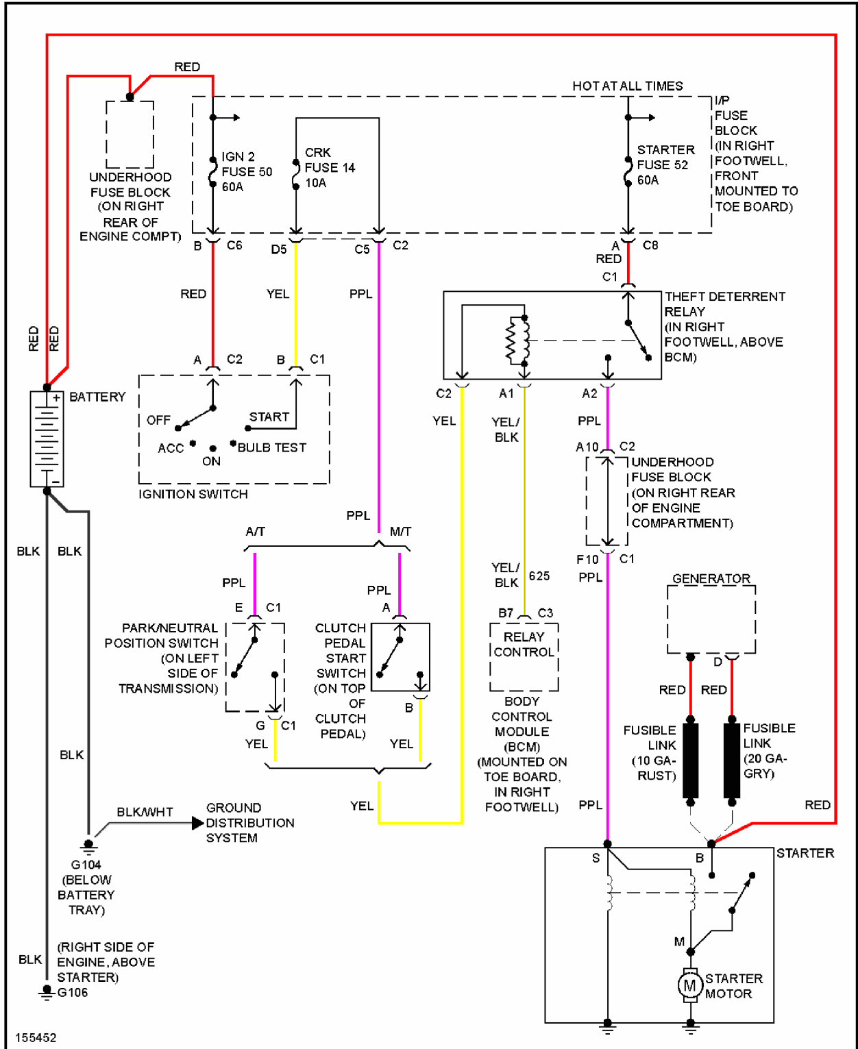
Fig. 44: Starting Circuit
