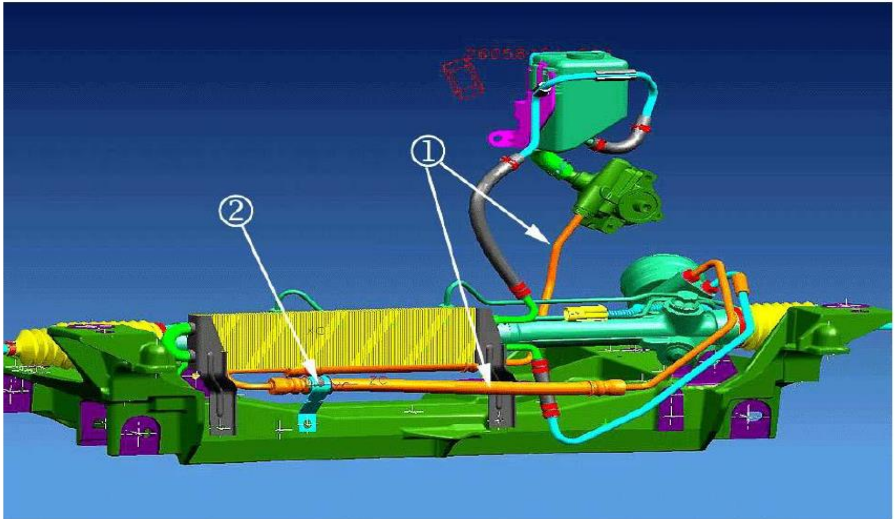
Fig. 2: Vehicles FE3 and FE4 Suspension Courtesy of GENERAL MOTORS CORP.
