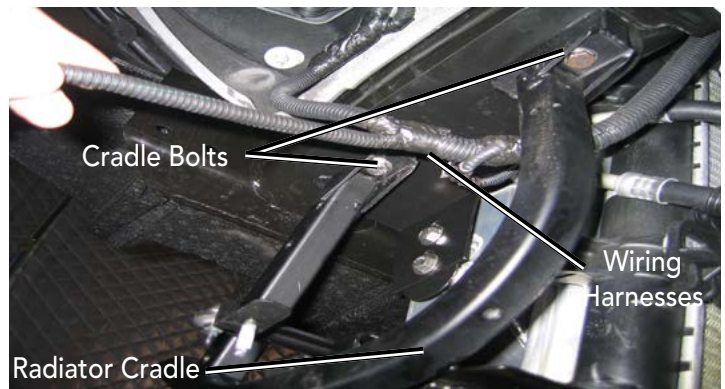
Factory Cradle Removal
