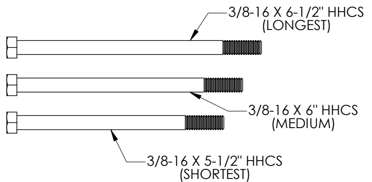
Bolt Lengths
