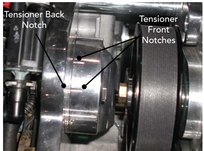
Belt Tensioning
