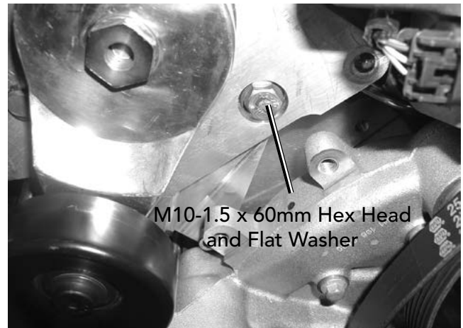
Sub-Bracket Mounting
