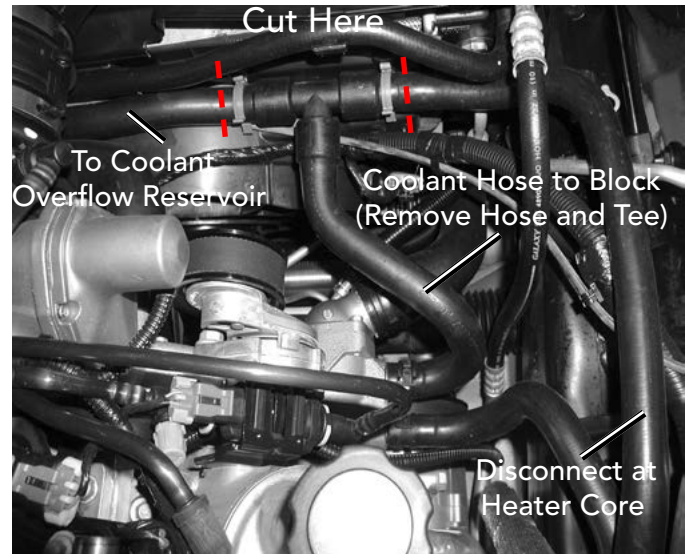
Coolant Hose Modification
