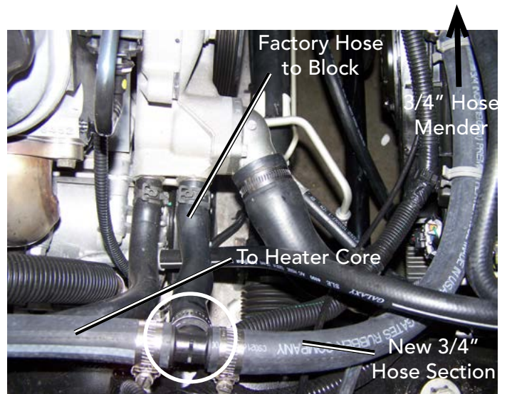
New Tee (Viewed from Passenger's Side)
