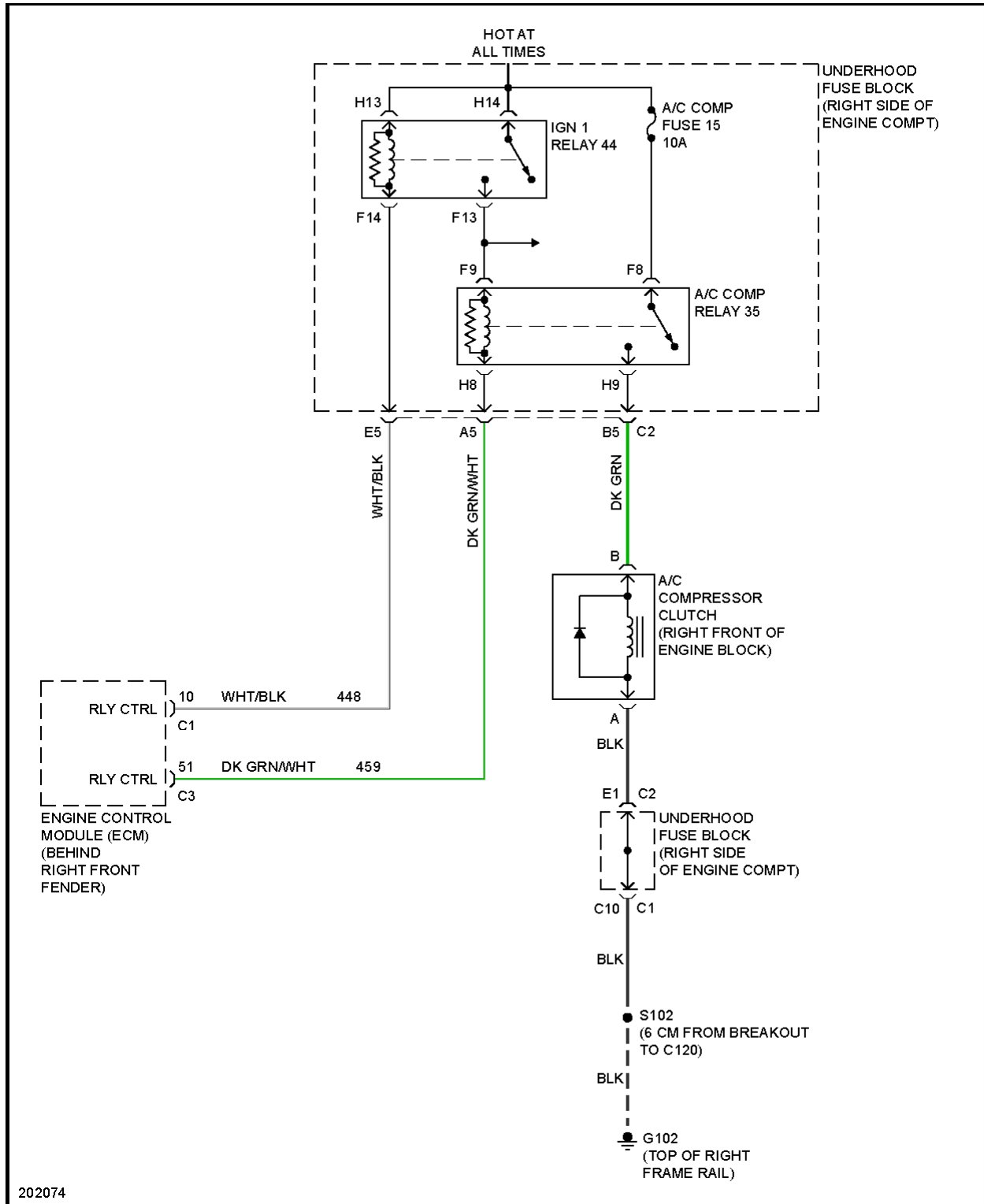
Fig. 3: Compressor Circuit
