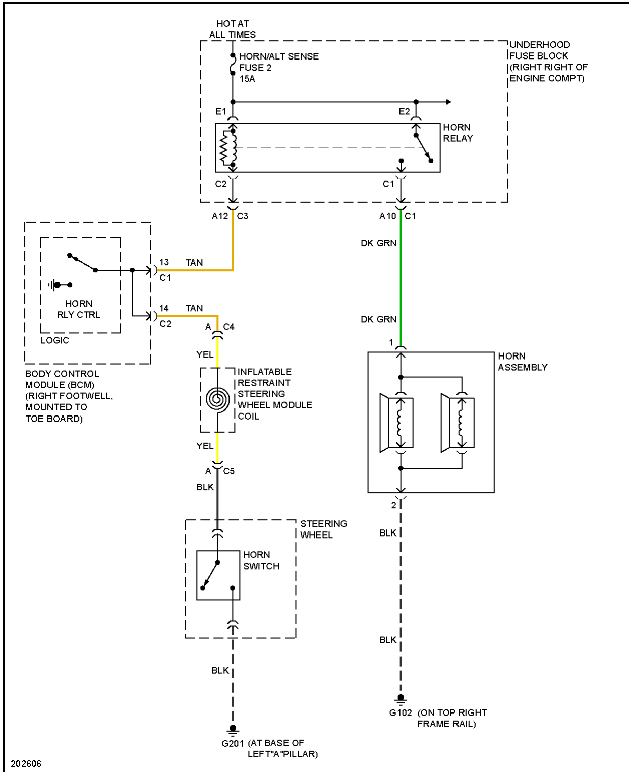
Fig. 35: Horn Circuit
