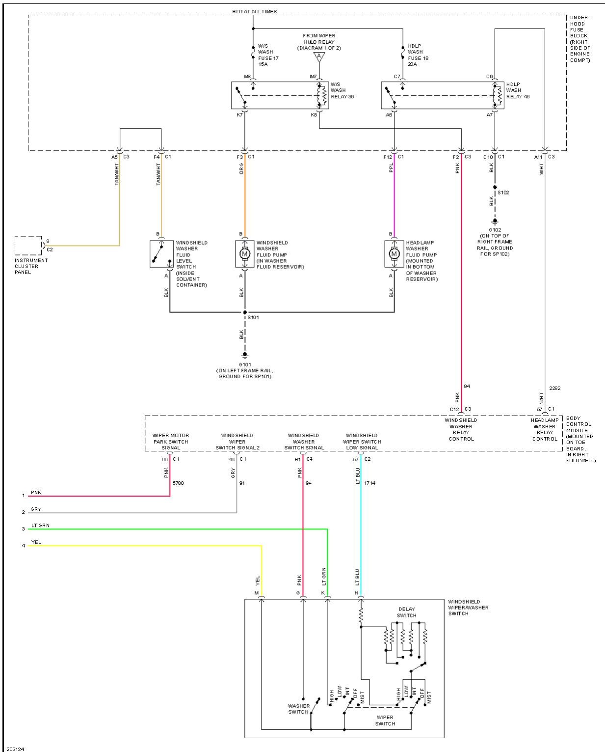
Fig. 72: Wiper/Washer Circuit (2 of 2)
