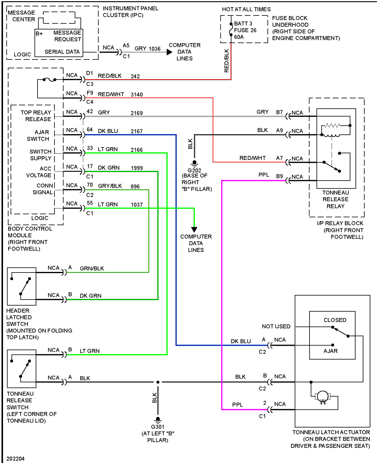
Fig. 55: Convertible Top Circuit, W/ Manual Top
